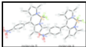
Fig. 1. Molecular structure of the title compound with the atom-numbering scheme. Displacement ellipsoids are drawn at the 30% probability level. Hydrogen atoms are omitted for clarity.
